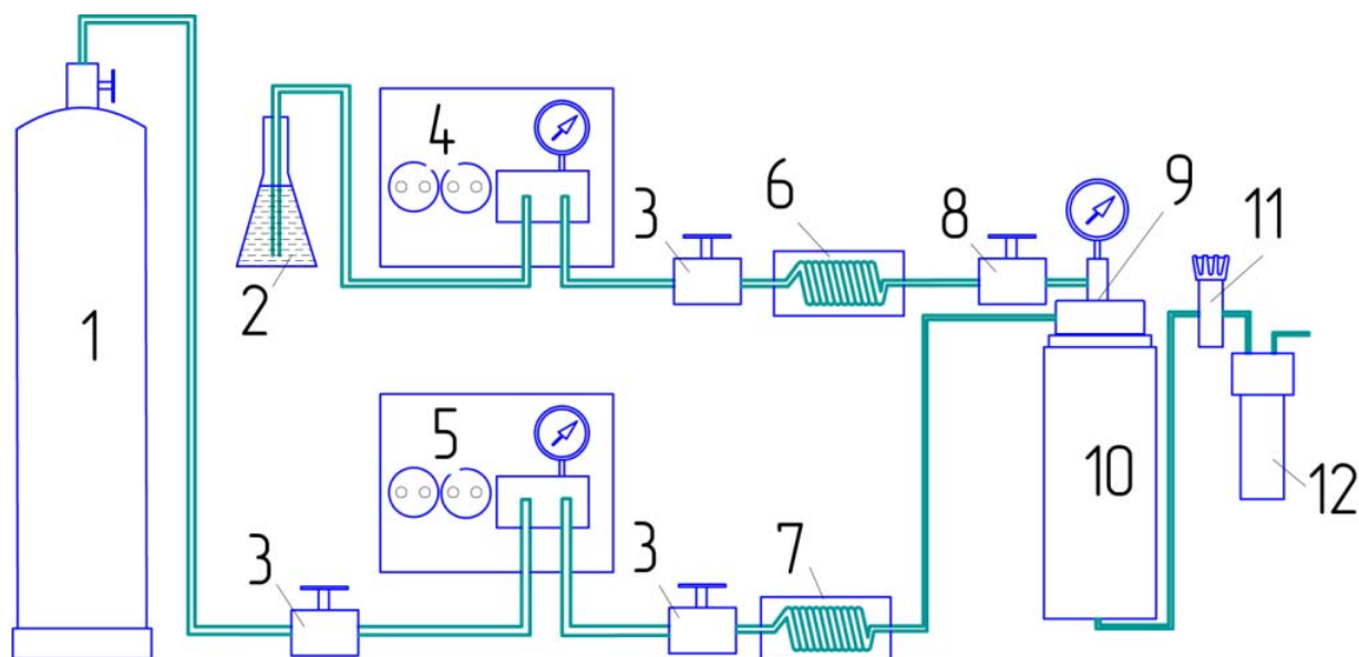
Fig. 1. Diagram of an experimental setup for dispersing polymer mixtures according to the SEDS method: 1 - CO 2 bottle, 2 - container for the "test substance - organic solvent" solution, 3 - valve, 4 - solution supply pump, 5 - CO 2 supply pump, 6 - solution heater, 7 - CO 2 heater, 8 - valve on the solution supply line to the nozzle, 9 - coaxial nozzle, 10 - reactor, 11 - back pressure regulator, 12 - separator.
