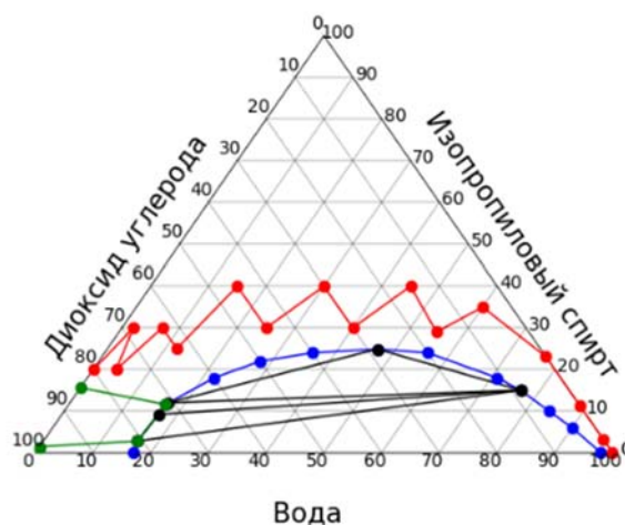
Fig. 1. Work line of the pressurized solvent exchange process on the ternary diagram of the “isopropyl alcohol - water - carbon dioxide” system
