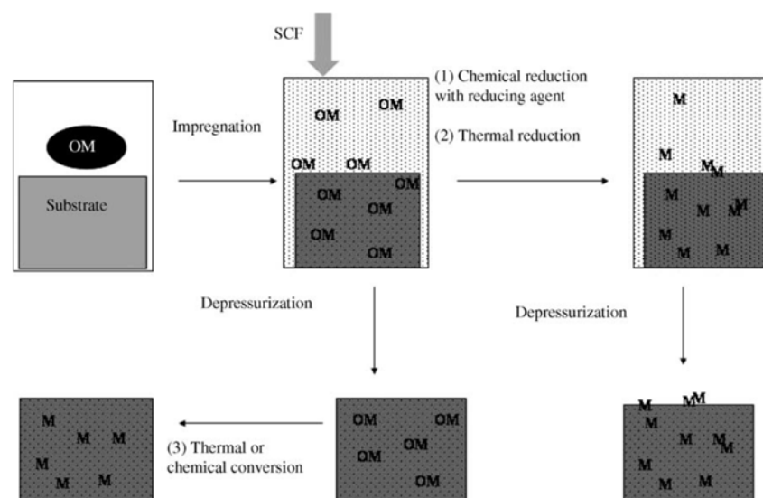
Figure. The scheme of using SCF as processing solvent to synthesize supported nanoparticles via deposition or impregnation; OM – metal containing compound; M – metallic particle
