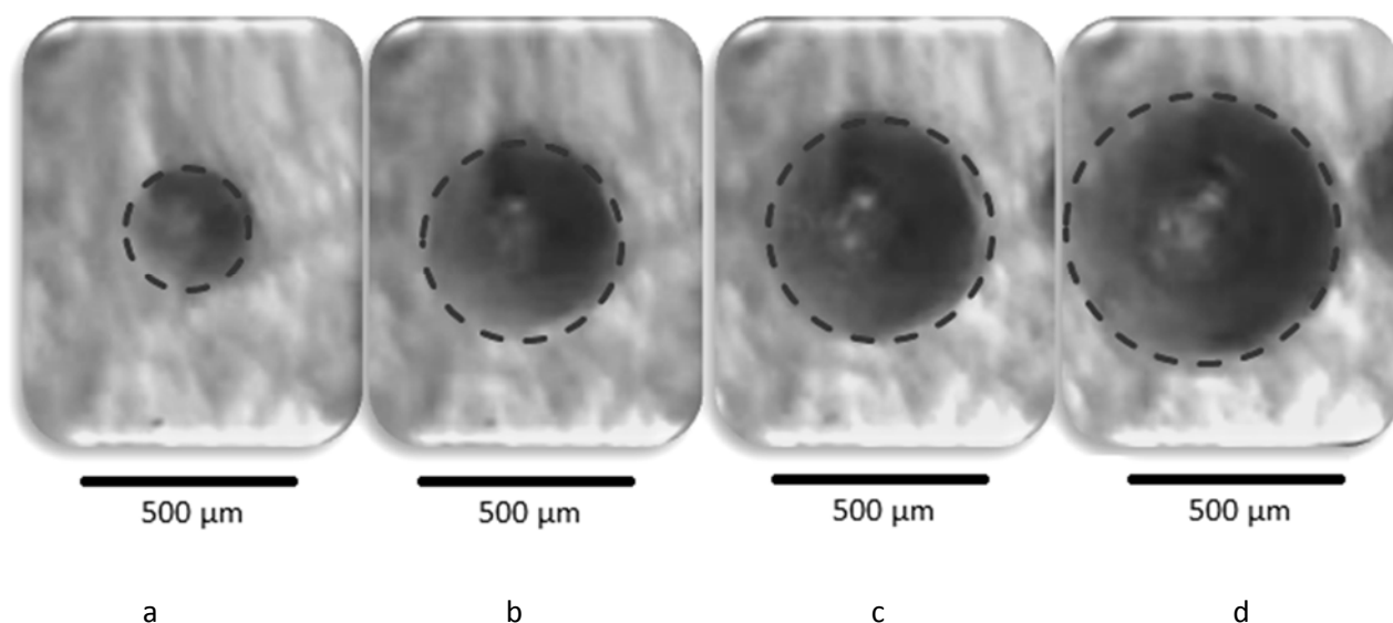
Figure 1. Dynamics of the stable growth of the single pore embryo in the foamed polylactide in the course of depressurization: P_{ext,0}=11.3\text{ MPa} , T=329\text{ K} , a) P_{ext}=9.05\text{ MPa} , R=80\text{ }\mu\text{m} , b) P_{ext}=8.86\text{ MPa} , R=140\text{ }\mu\text{m} , c) P_{ext}=8.72\text{ MPa} , R=160\text{ }\mu\text{m} , d) P_{ext}=8.53\text{ MPa} , d=210\text{ }\mu\text{m} .
