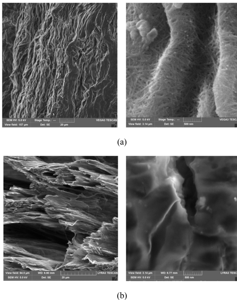
Fig. 1. SEM images of NCC samples obtained by drying in supercritical carbon dioxide (a) and by freeze drying (b)
