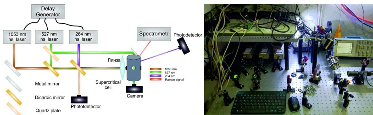
Fig. 1. System for time-resolved diagnostics of extreme state of matter in sc-CO 2 .
