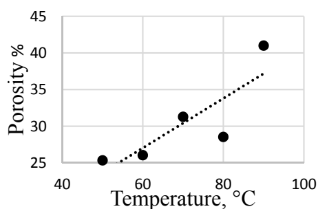
Figure: 1 Dependence of PLA porosity on temperature
