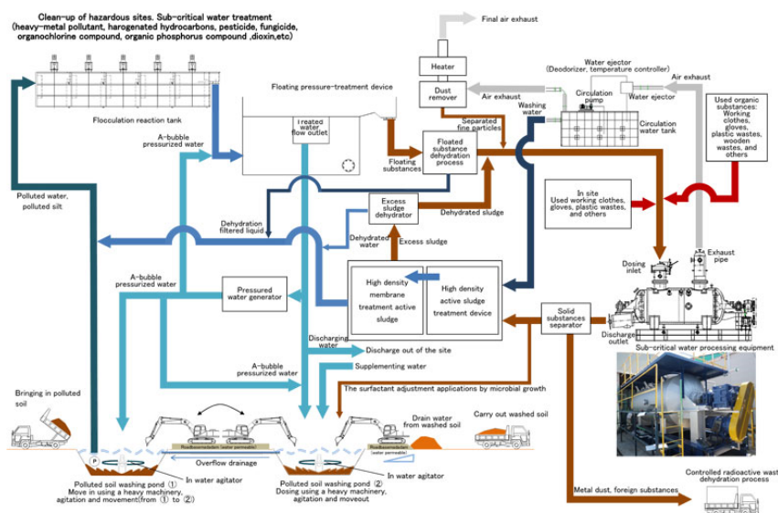
Fig. 3. SRIC System.
