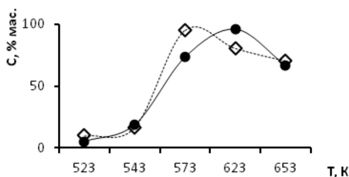
Figure: 1. Temperature dependence of oleic acid content at volumetric ratios (water: rapeseed oil):
