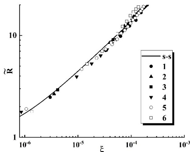
Fig. 1. Self-similar nature of the dependences of the embryos radii in polylactide matrices on external pressure: the dependences obtained at different values of the initial pressure P_{ext}^{in} and temperature T are reduced to a universal function ( s-s ) by linear transformations of coordinates.
